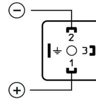
right-angle plug
