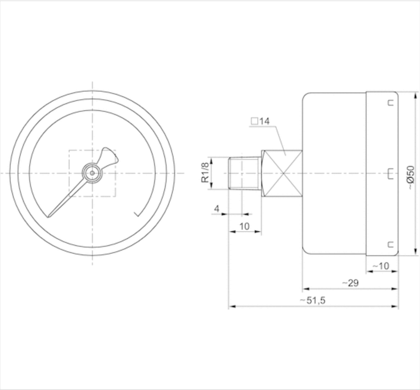
Dimensions, Fig. 2, Safety glass viewing window
