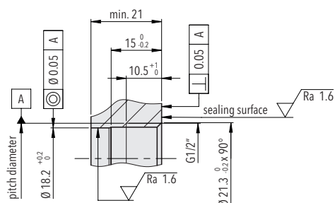
Mounting thread G1/2" DIN EN ISO 1179-1
