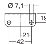
Mounting brackets
