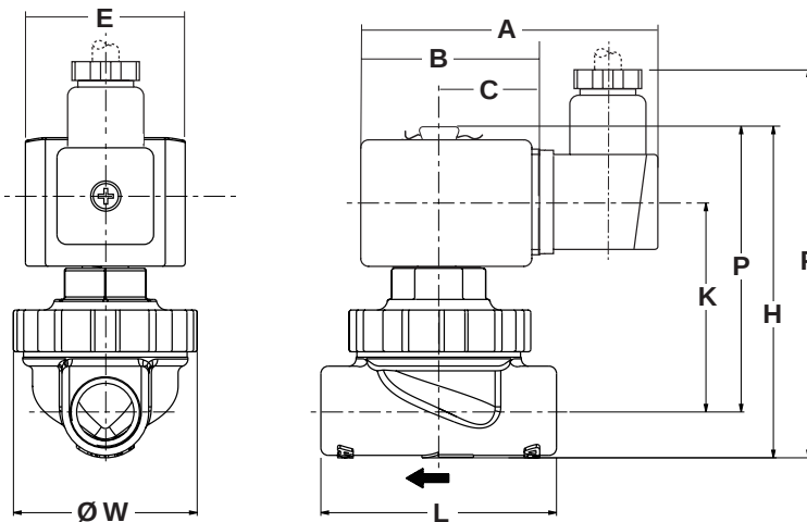
TYPE 01 Electrical interface "S1" Epoxy moulded IEC 335 / ISO 4400 IP65
