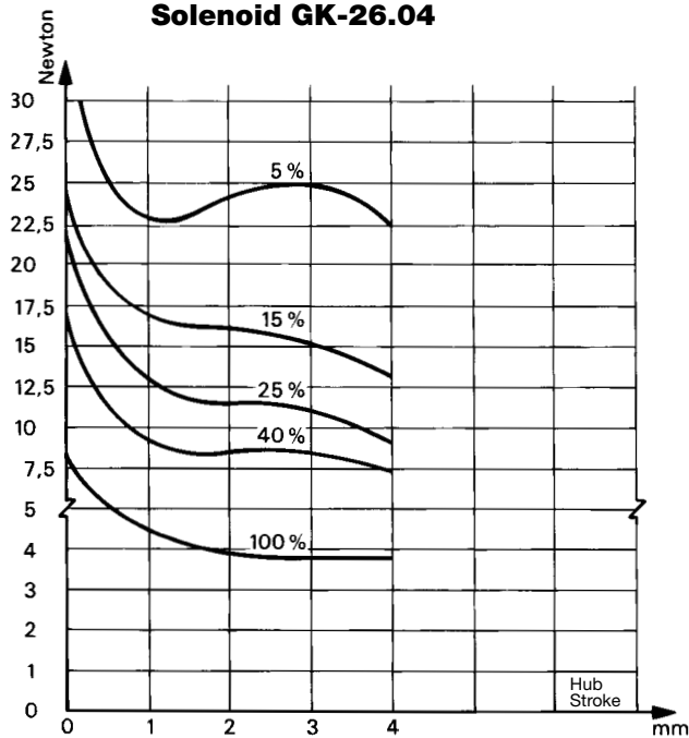
Magnettyp GK-26.04 Solenoid GK-26.04
