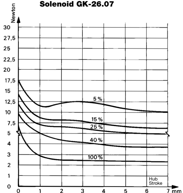
Magnettyp GK-26.07 Solenoid GK-26.07
