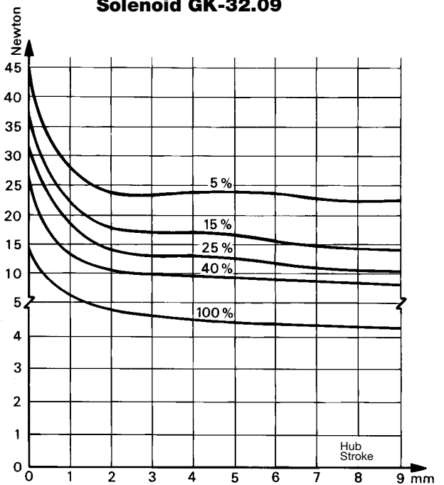
Magnettyp GK-32.09 Solenoid GK-32.09
